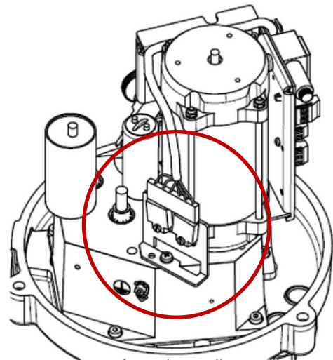
Abbildung 2: Verschraubung externe Relais PSL320-PSL330 / Figure 2: Screw fitting external relays PSL320-PSL330
