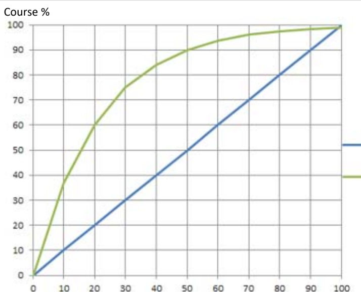
Figure 11: Courbe de la valve
